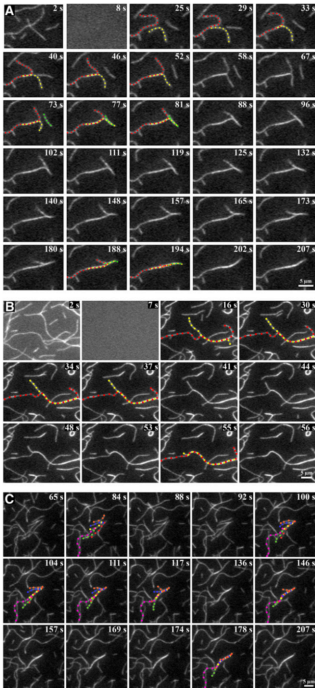
Figure 4. Time-Lapse TIRFM Allows Real-Time Visualization of Bundle Formation by Villins In Vitro .
