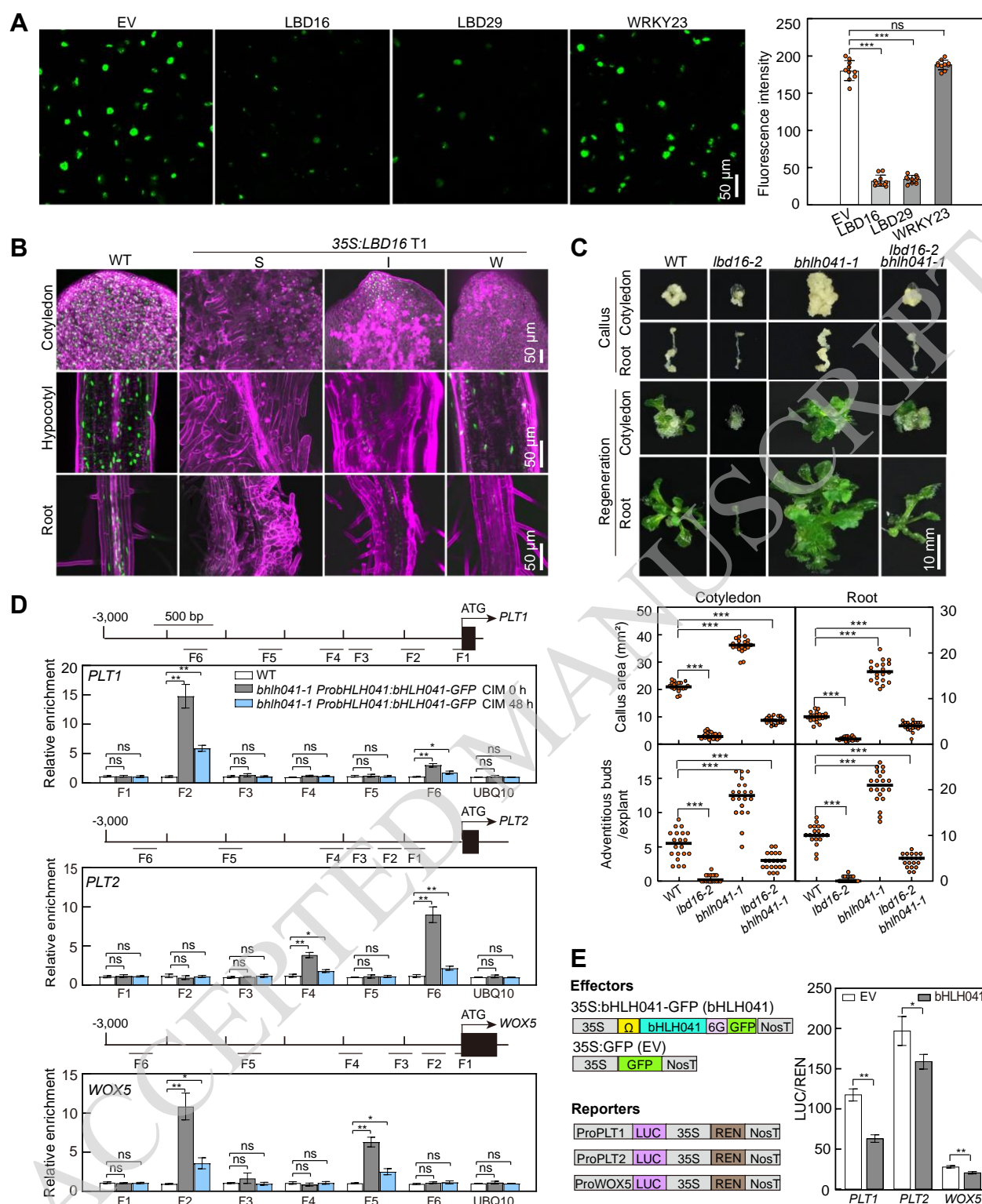
Figure 5. LBD induces the removal of bHLH041 to alleviate bHLH041-mediated repression of PLT1 , PLT2 and WOX5 transcription.
