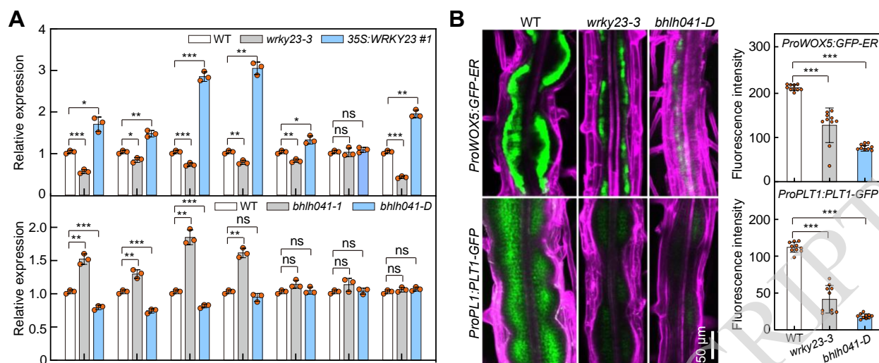
Figure 3. WRKY23 and bHLH041 are activator and repressor of root stem cell genes, respectively.
