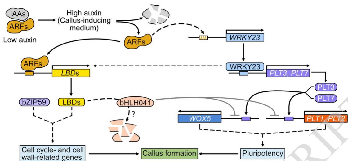
Figure 7. A proposed molecular framework for auxin-induced callus formation.
