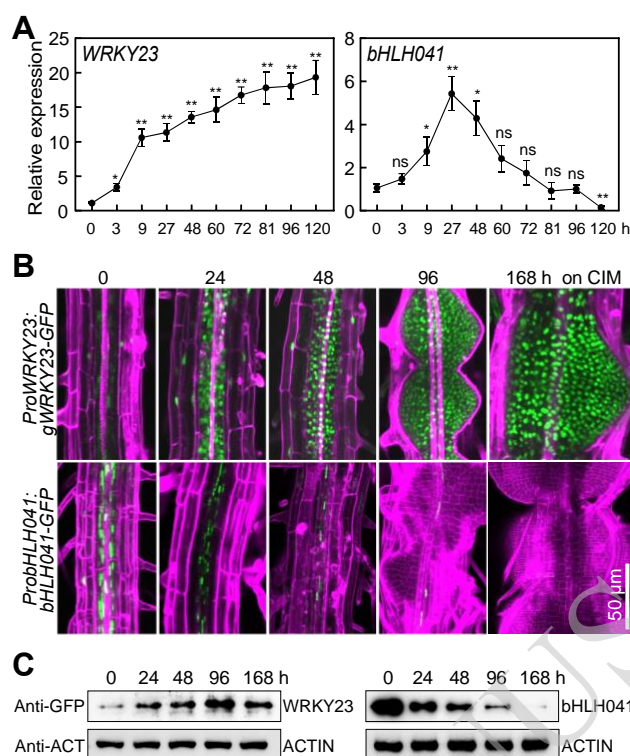
Figure 1. Accumulation of WRKY23 and bHLH041 during callus induction.
