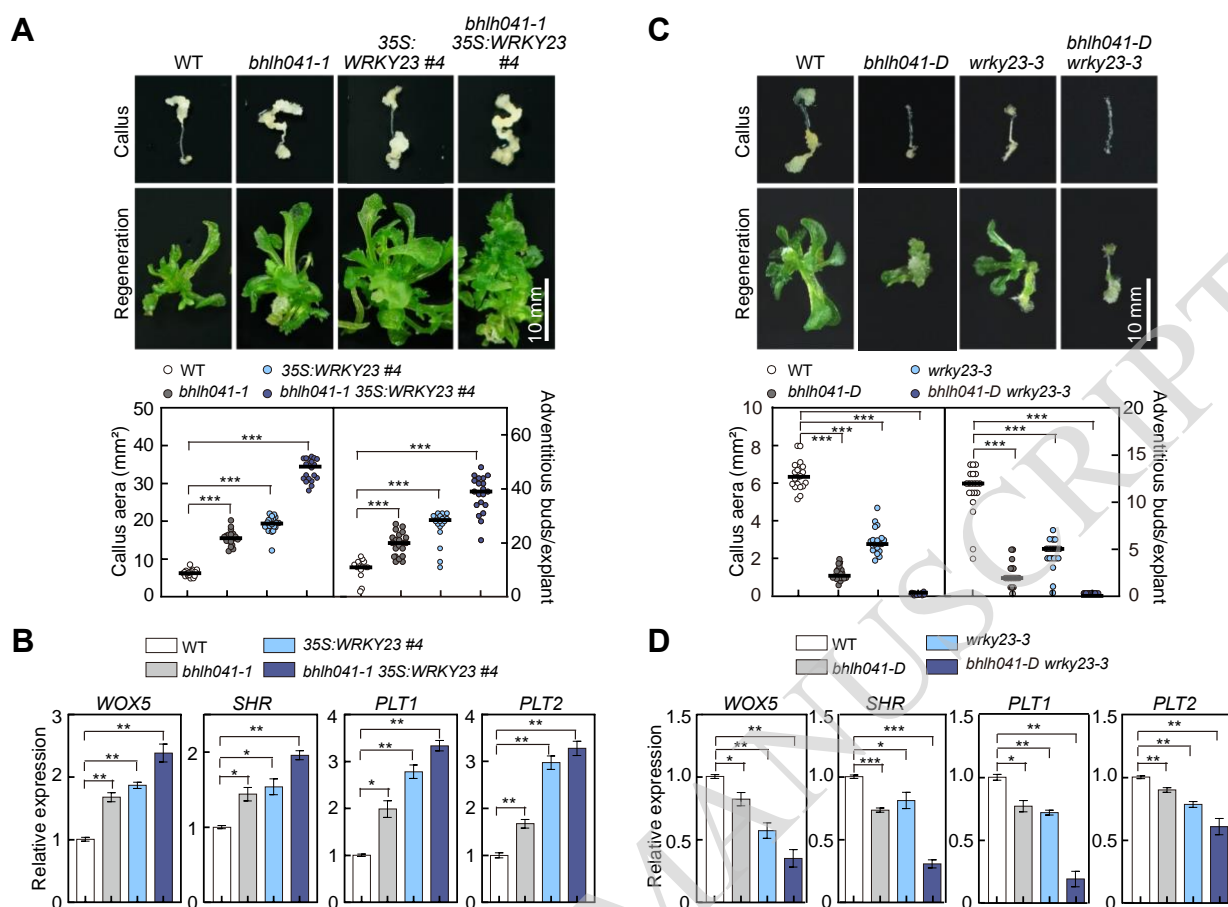
Figure 6. WRKY23 and bHLH041 synergize shoot-regenerating capability of callus.
